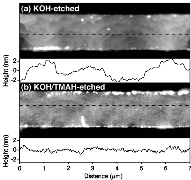
FIG. 2. AFM images and line scans of etched beams. (a) A 4 min KOH etch leads to a macrostep-covered surface (1.5 nm rms), and (b) a 3 min KOH etch followed by a 4 min TMAH etch leads to smooth surfaces (0.4 nm rms).
