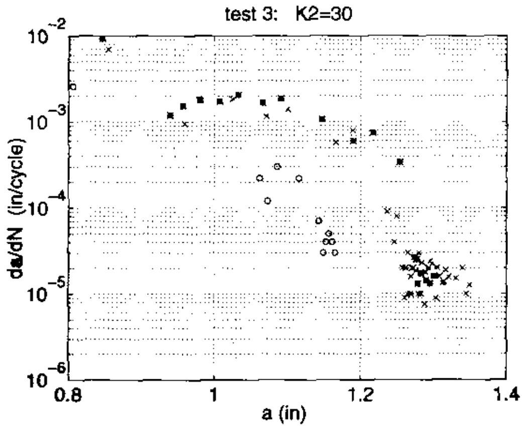
Figure 7 , Mixed-mode fatigue crack growth rate vs. crack length from constant DK_1 , DK_2 tests. Initial crack length is 0.8 inches.
