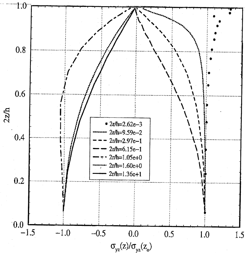
Figure 4, Thin cracked plate under uniform shear ( h/a=0.02 ). Distributions of the out-of-plane shear stress through the thickness from a three dimensional finite element analysis at different radial distances from the crack tip. ( z_0=0.065 h/2 )
