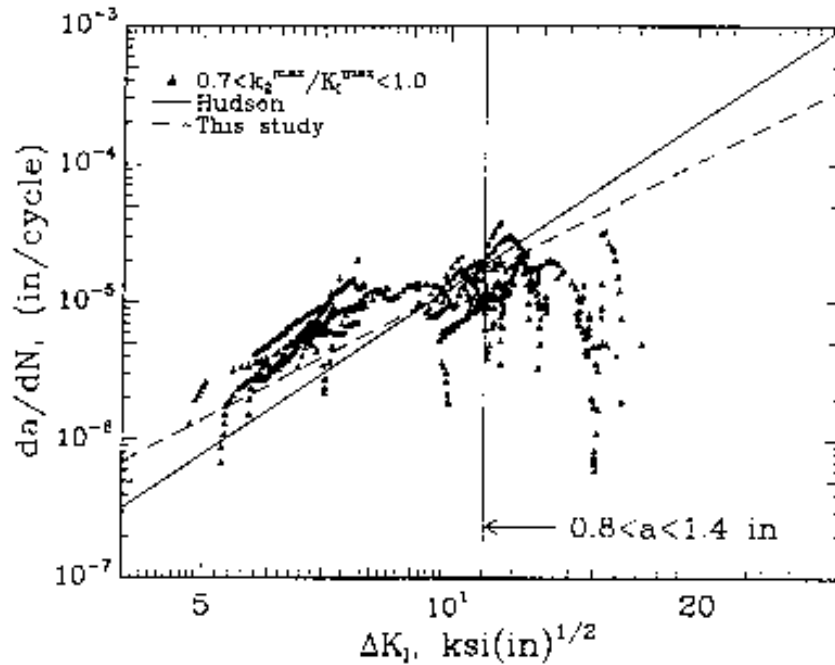
Figure 6, Mixed-mode fatigue crack growth rate results from relatively large values of Dk_2 . The solid and dashed lines represent the crack growth rate for pure mode-I loading. The vertical line indicates the range of crack lengths present in this data when DK_I = 11 \text{ ksi in}^{1/2} .
