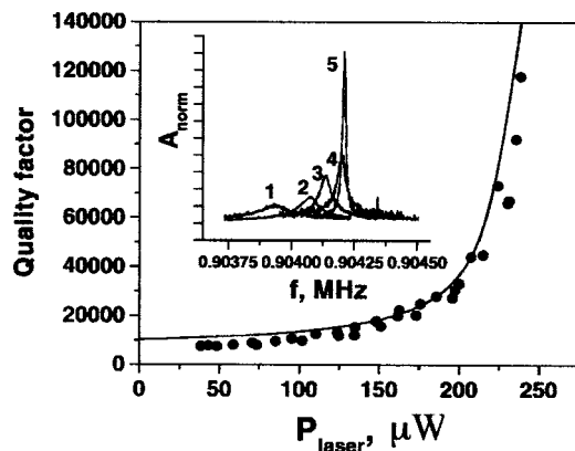
FIG. 2. Quality factor of the disk oscillator ( 40 \mu\text{m} outer diameter and 6.7 \mu\text{m} \text{SiO}_2 pillar diameter) as a function of the CW laser power is shown. Light intensity was kept below the self-generation threshold, while the oscillations were driven by a piezotransducer. Solid line represents the result of theoretical calculations. Inset shows the shape of the spectra acquired for different values of laser power: 58 \mu\text{W} (line 1), 124 \mu\text{W} (line 2), 162 \mu\text{W} (3), 198 \mu\text{W} (4), and 235 \mu\text{W} (5) (the curves are normalized by the light intensity and the piezovoltage).
